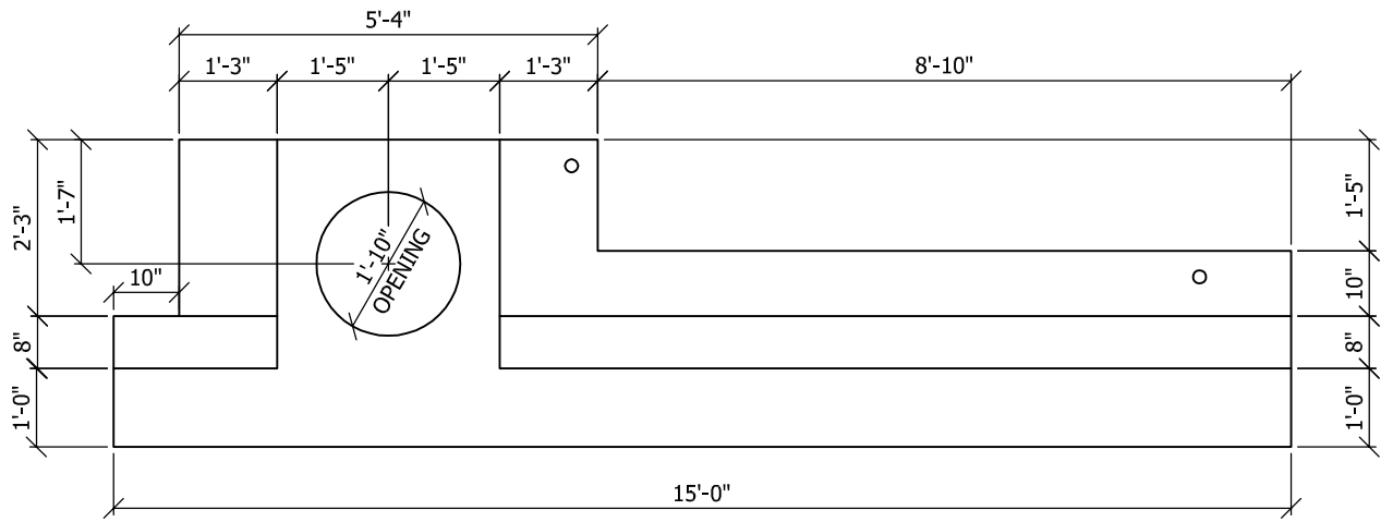
REINFORCED CONCRETE COVER FOR CURB INLET. TYPE I, II, & III
