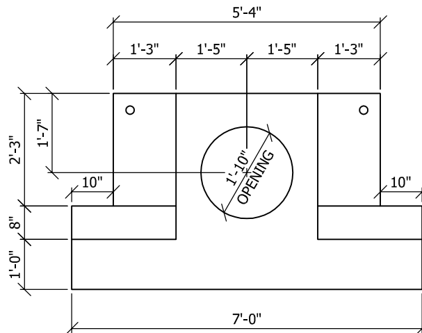
REINFORCED CONCRETE COVER FOR CURB INLET. TYPE IV
