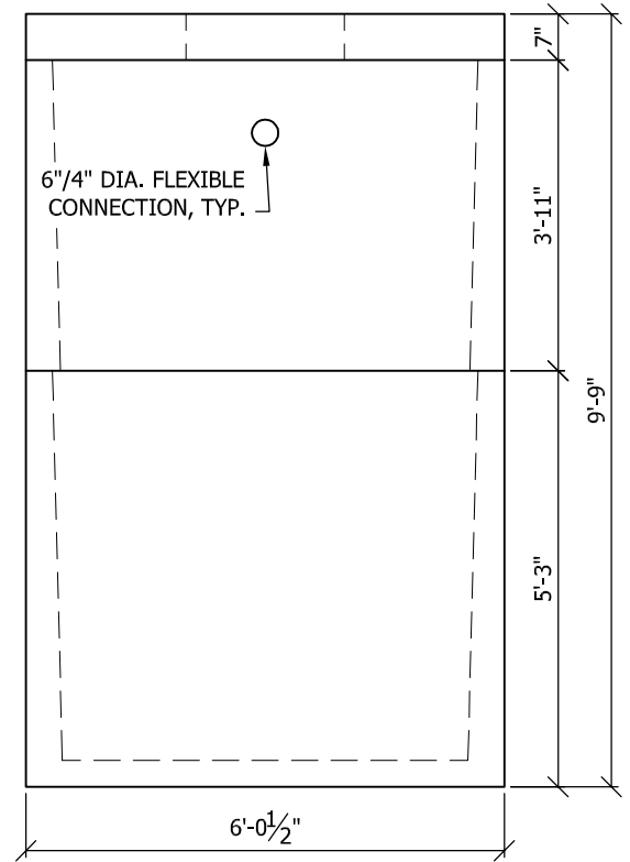
END VIEW
