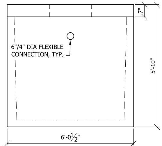
END VIEW
