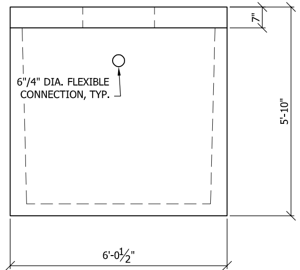
END VIEW
